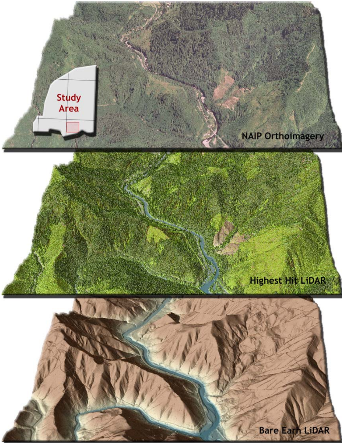
Figure 322. 3-d oblique view of LiDAR-derived surfaces in 7.5' Quad 45123D6, showing Wilson River near the Little North Fork confluence in the ODF South study area.
