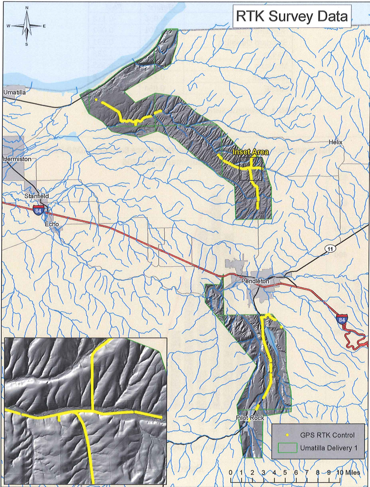
Figure 6. Locations of RTK control surveyed by DOGAMI. Data was used to test absolute accuracy for the Umatilla lidar survey within the Delivery 1 extent.
