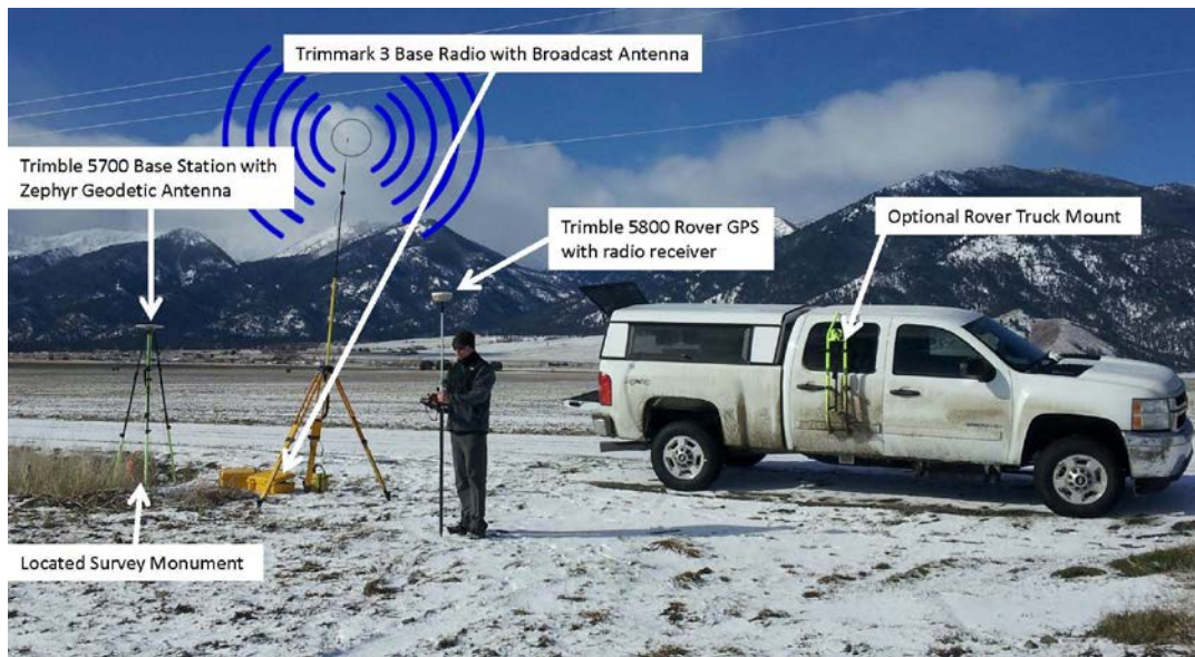
Figure 5. The Trimble 5700 base station antenna located over a known reference point near Cove, OR. Corrected GPS position and elevation information is then transmitted by a Trimmark III base radio to the 5800 GPS rover unit.
