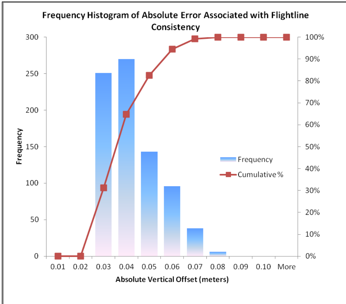
Figure 2. LiDAR Flight line Consistency Error Distribution
