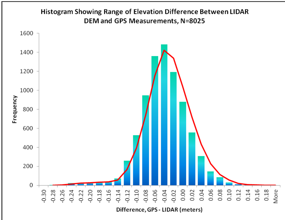
Figure 7. Distribution of LiDAR Vertical Error
