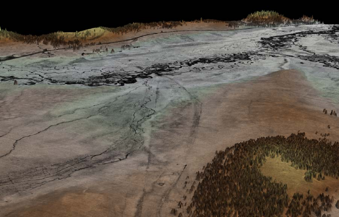
Figure 11. View looking North across the Grande Ronde Basin at the confluence of Sheep Creek and the Grande Ronde River. Images derived from a gridded surface of LiDAR points colored by height.
