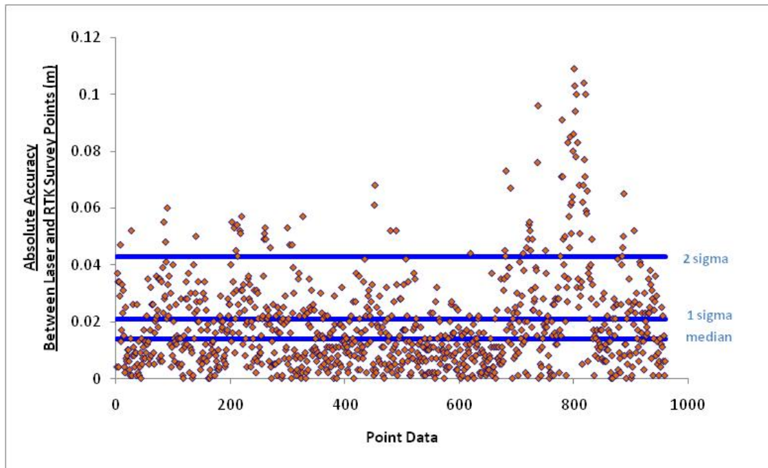
Figure 8. Absolute Accuracy - Absolute Deviation, based on hard surface points
