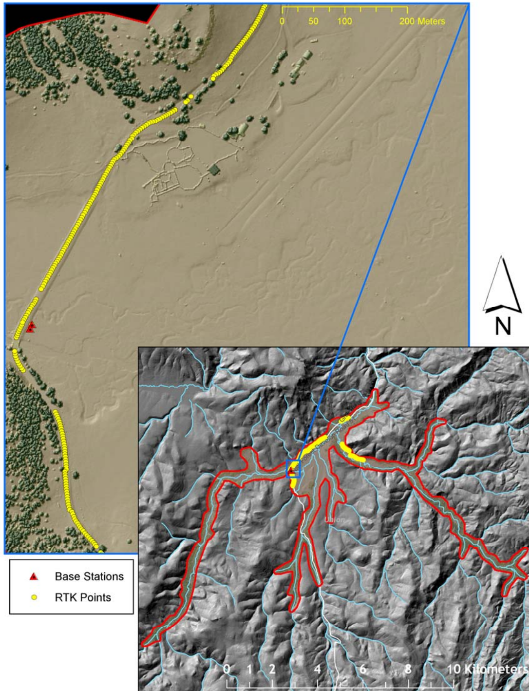
Figure 2. RTK and base station locations used for the Upper Grande Ronde River survey area overlaid on 10-m hillshade (bottom) and LiDAR derived highest-hit model (top).
