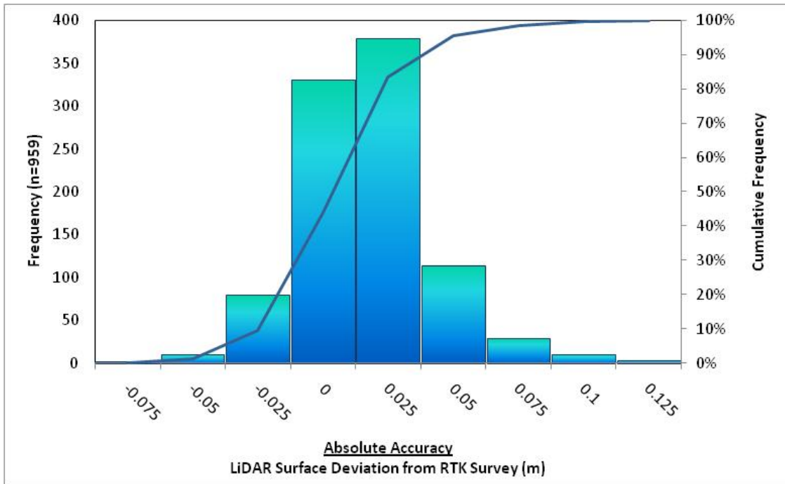
Figure 7. Absolute Accuracy - Histogram Statistics, based on hard surface points
