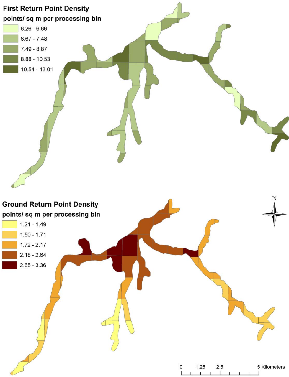
Figure 3. Density distribution for first-return and ground-classified laser point densities per processing tile.
