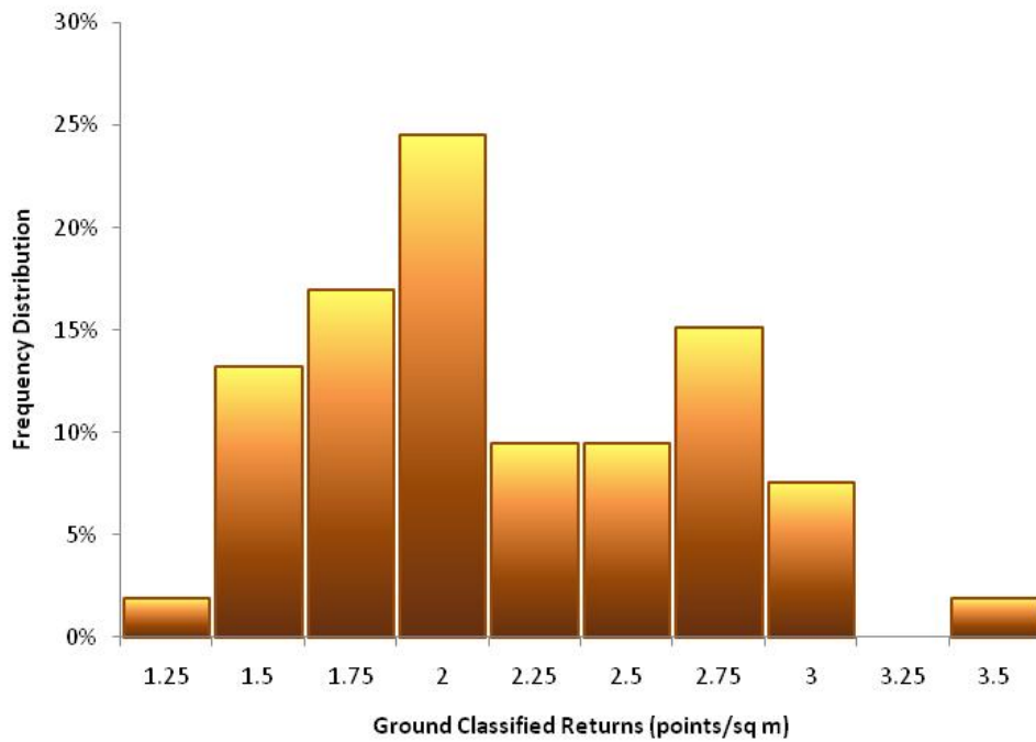
Figure 5. Density distribution for ground-classified laser points
