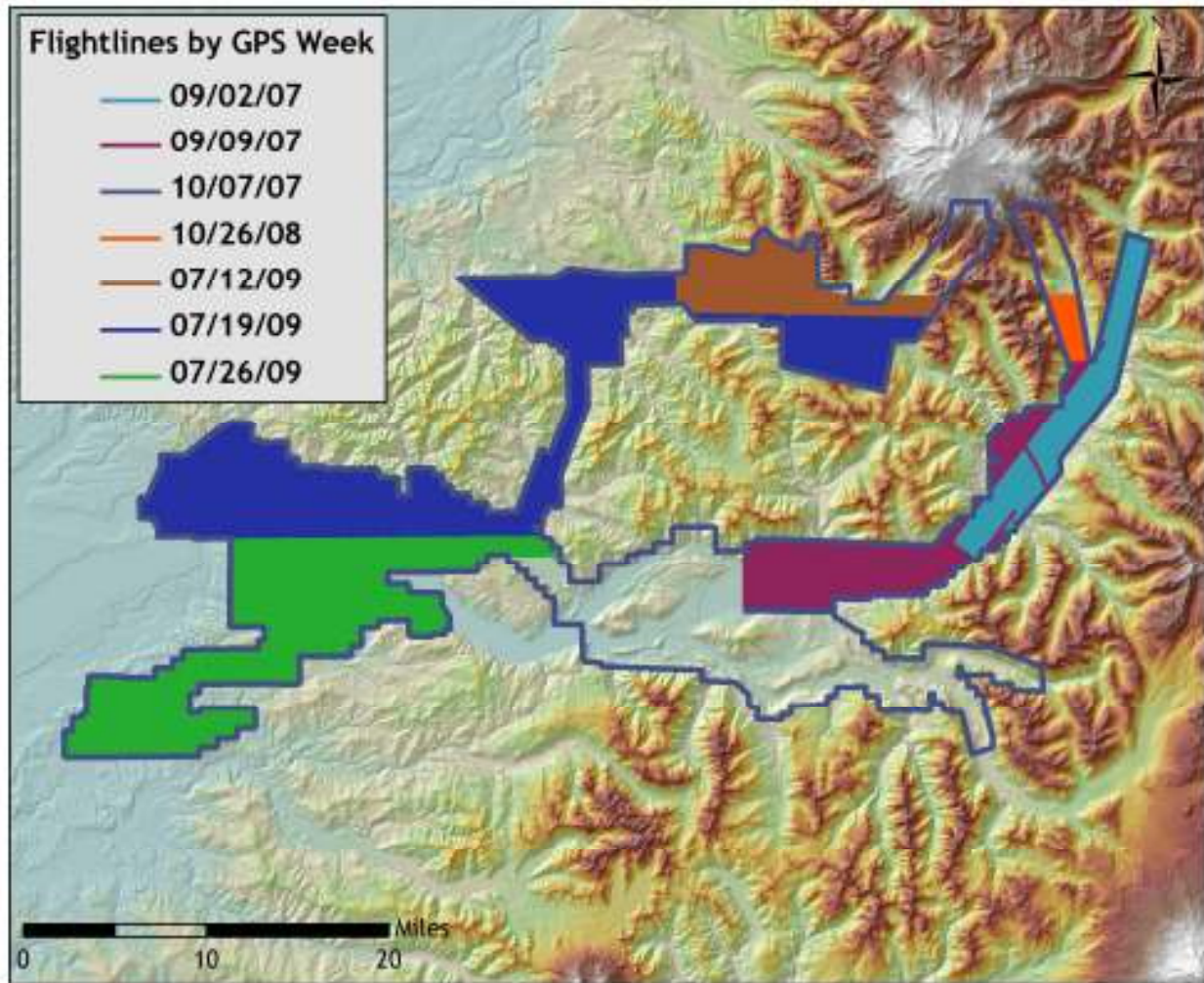
Figure 2.1. Completed flight lines (n=666) in Lewis County for area delivered to date.
