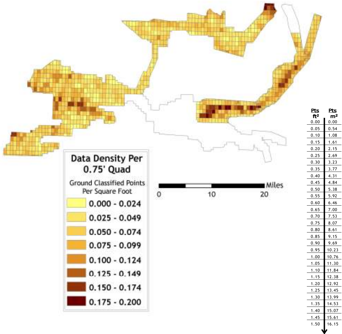
Figure 4.10. Image shows ground-classified laser point density for data delivered to date in the Lewis County study area, per 0.75' USGS Quad.
