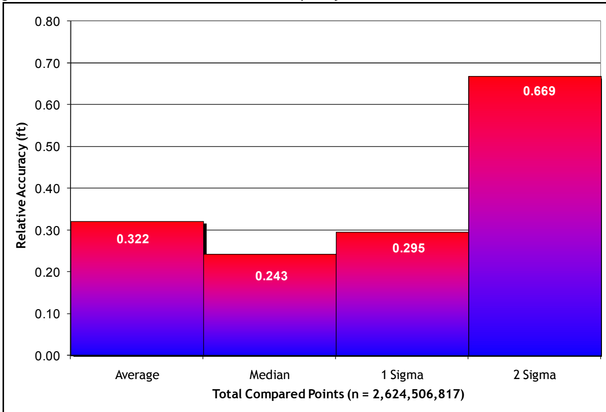
Figure 4.3. Statistical relative accuracies, non slope-adjusted.
