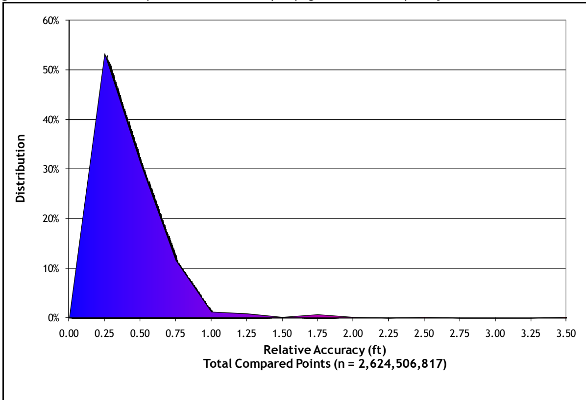
Figure 4.3. Statistical relative accuracies, non slope-adjusted.
