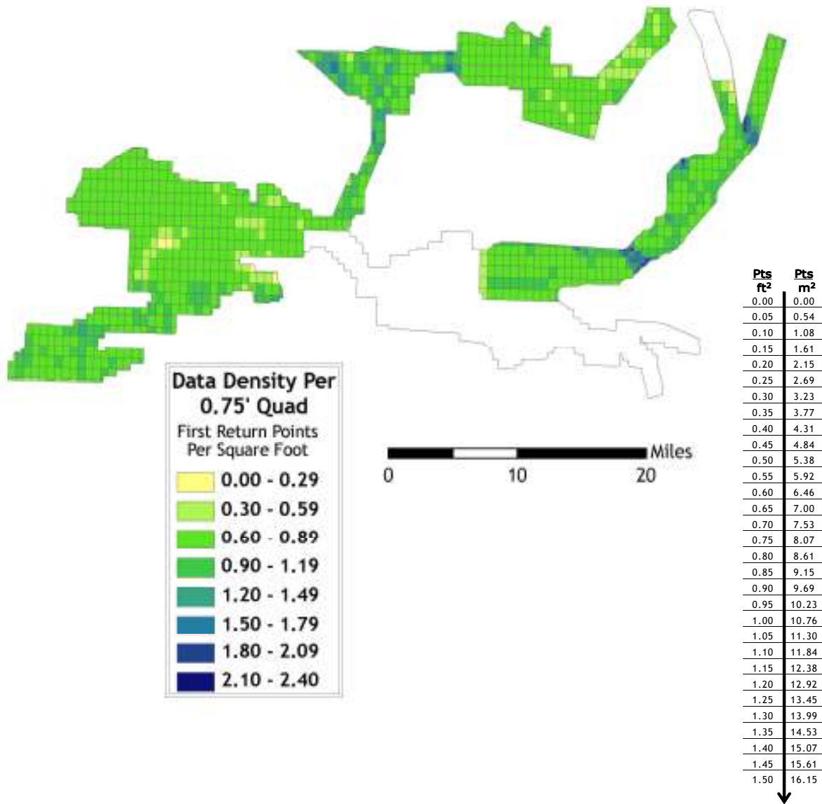
Figure 4.8. Image shows first return laser point density for data delivered to date in the Lewis County study area, per 0.75' USGS Quad.
