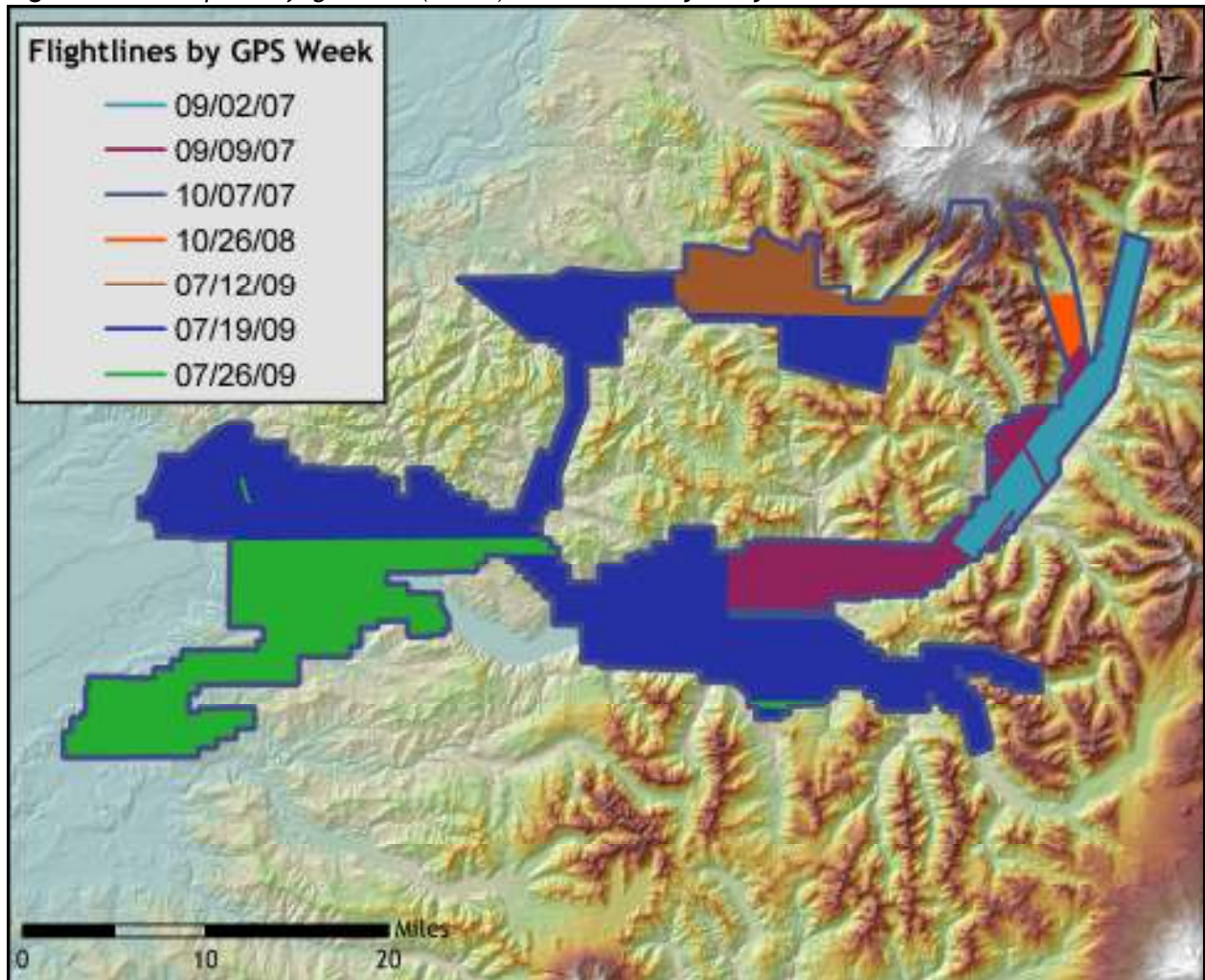
Figure 2.1. Completed flight lines (n=767) in Lewis County study area.
