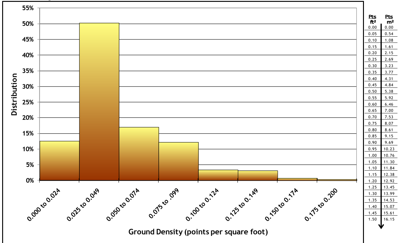
Figure 4.9. Histogram of ground-classified laser data density for in the Lewis County study area, per 0.75' USGS Quad.
