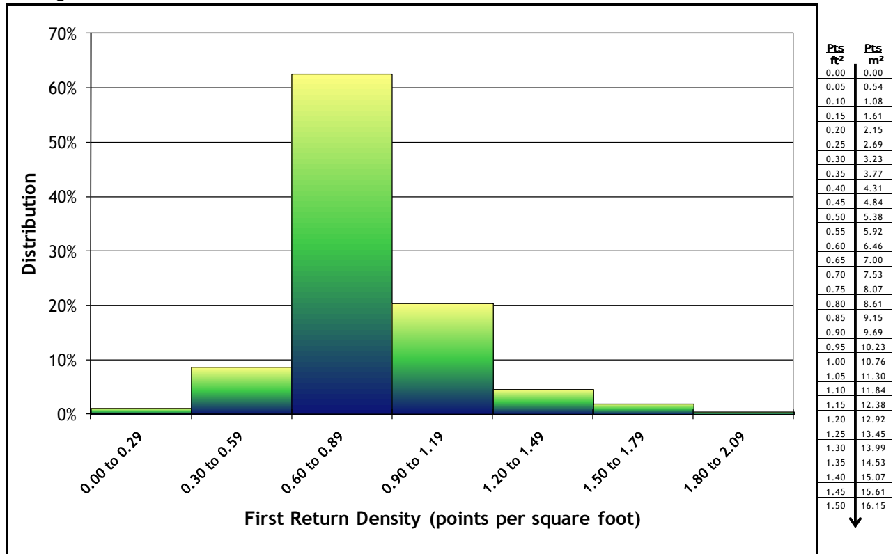
Figure 4.7. Histogram of first return laser point density for in the Lewis County study area, per 0.75' USGS Quad.
