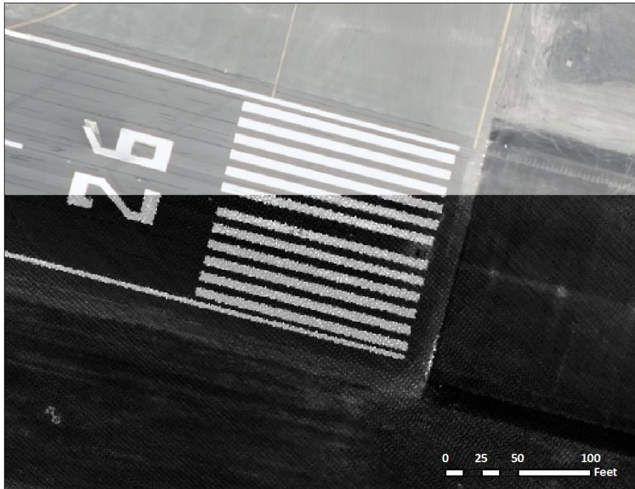
Figure 17: Image displaying the co-registration between the LiDAR intensity image and the 15 cm orthophoto at a location within the Juneau Priority 1 area.
