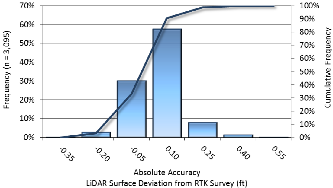
Figure 13: Frequency histogram for LiDAR surface deviation from RTK values
