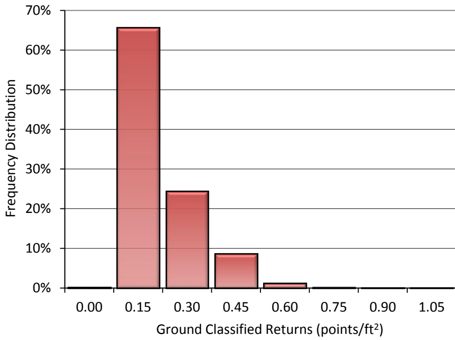
Figure 9: Frequency distribution of ground return densities of Priority Area 1
