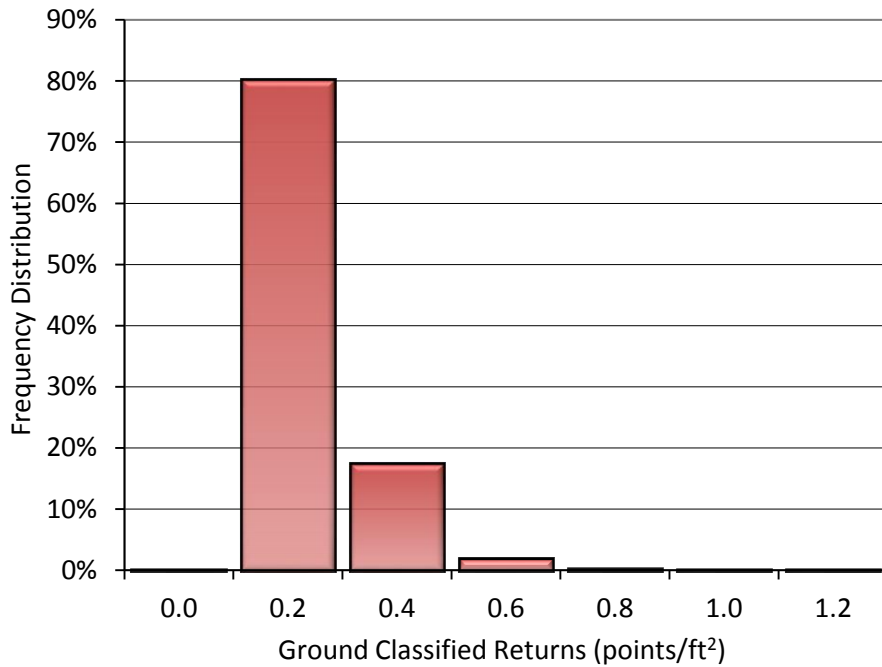
Figure 10: Frequency distribution of ground return densities of Priority Areas 2 and 3
