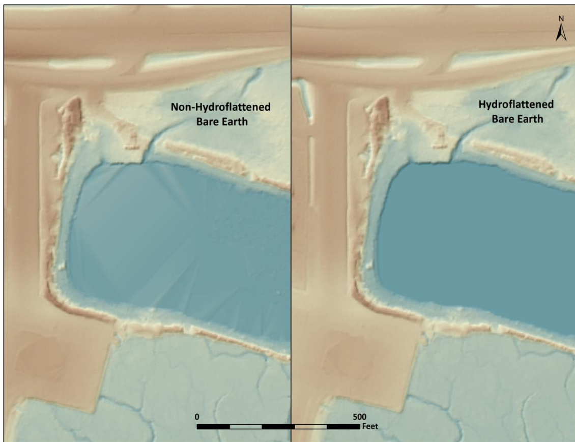
Figure 6: Example of hydro-flattening in the Juneau LiDAR dataset
