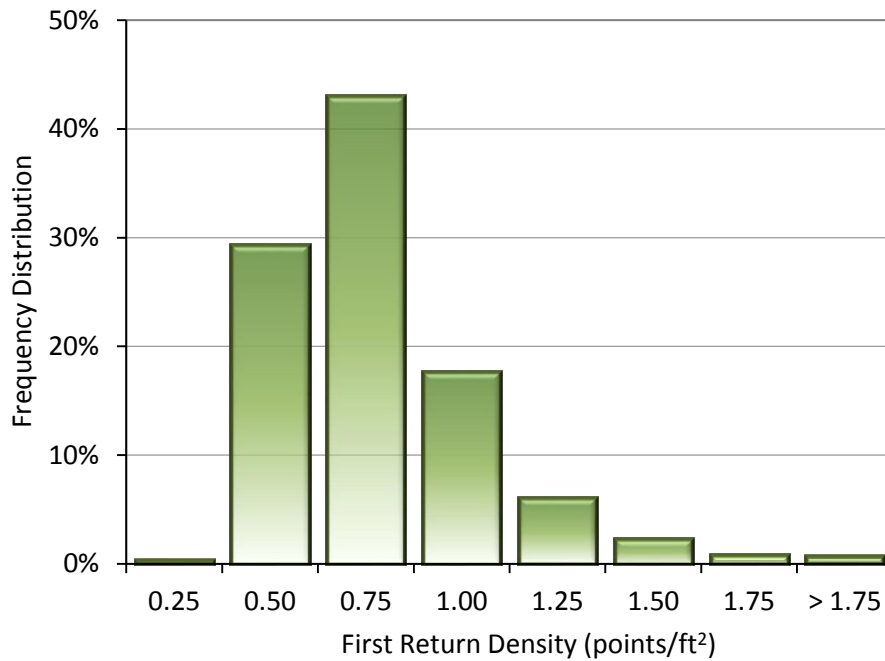
Figure 8: Frequency distribution of first return densities (native densities) of Priority Areas 2 and 3
