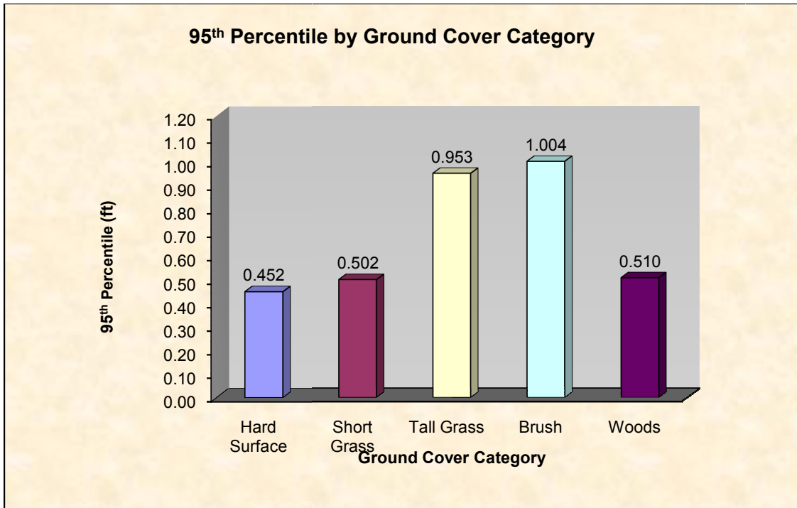
Figure 1: Graph of SVA Values by Ground Cover Category
