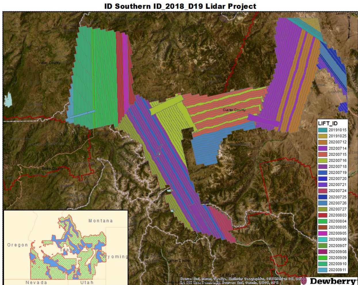
Figure 3. WUID 300076 swaths
