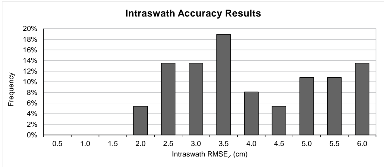
Figure 10. Frequency distribution of intraswath RMSD z results for WUID 300076
