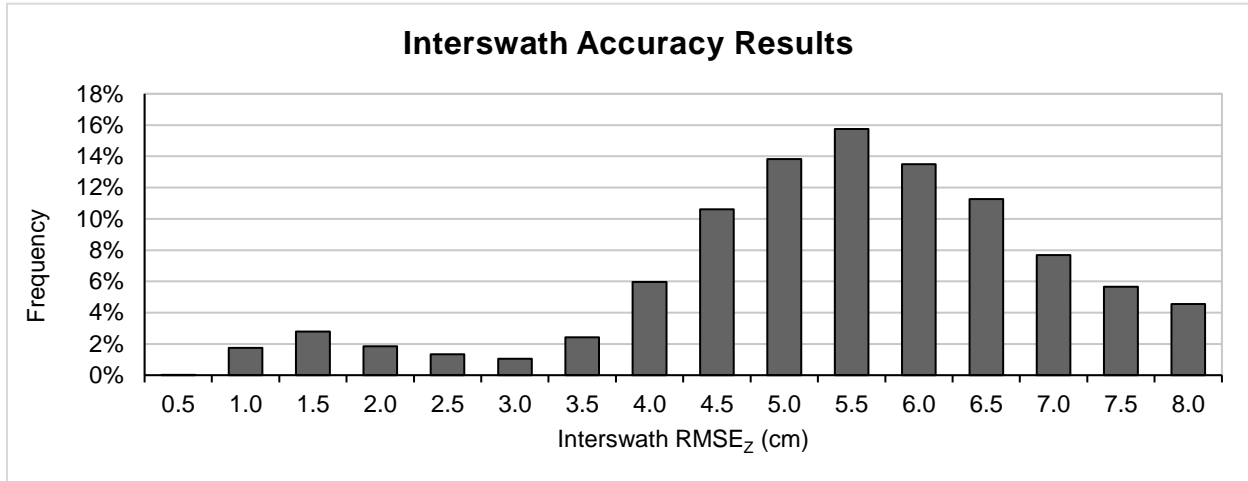
Figure 7. Frequency distribution of interswath RMSDz results for WUID 300076
