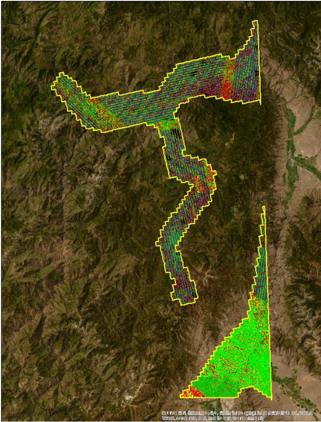
Figure 5. Swath Separation Images (SSIs) generated for WUID 300226.
