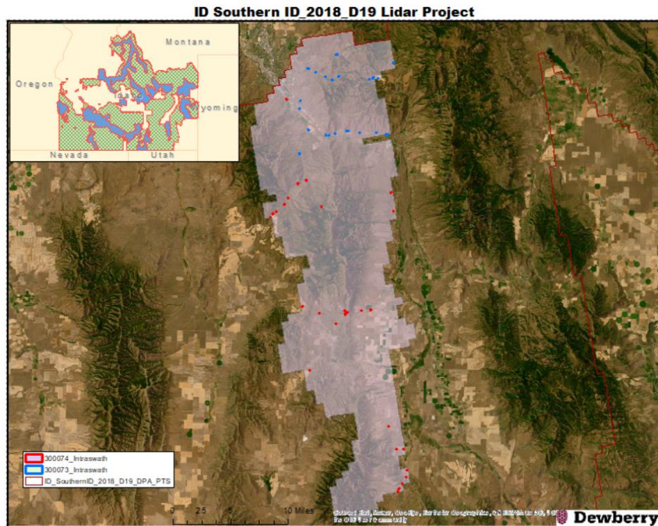
Figure 8. Intraswath polygons used to test intraswath vertical accuracy.
