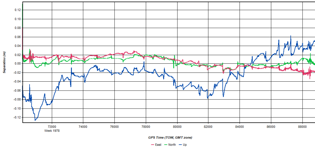
Figure 3: W_Central_3DEP_20171203_192639 [Smoothed TC Combined] - Forward/Reverse or Combined Separation Plot
