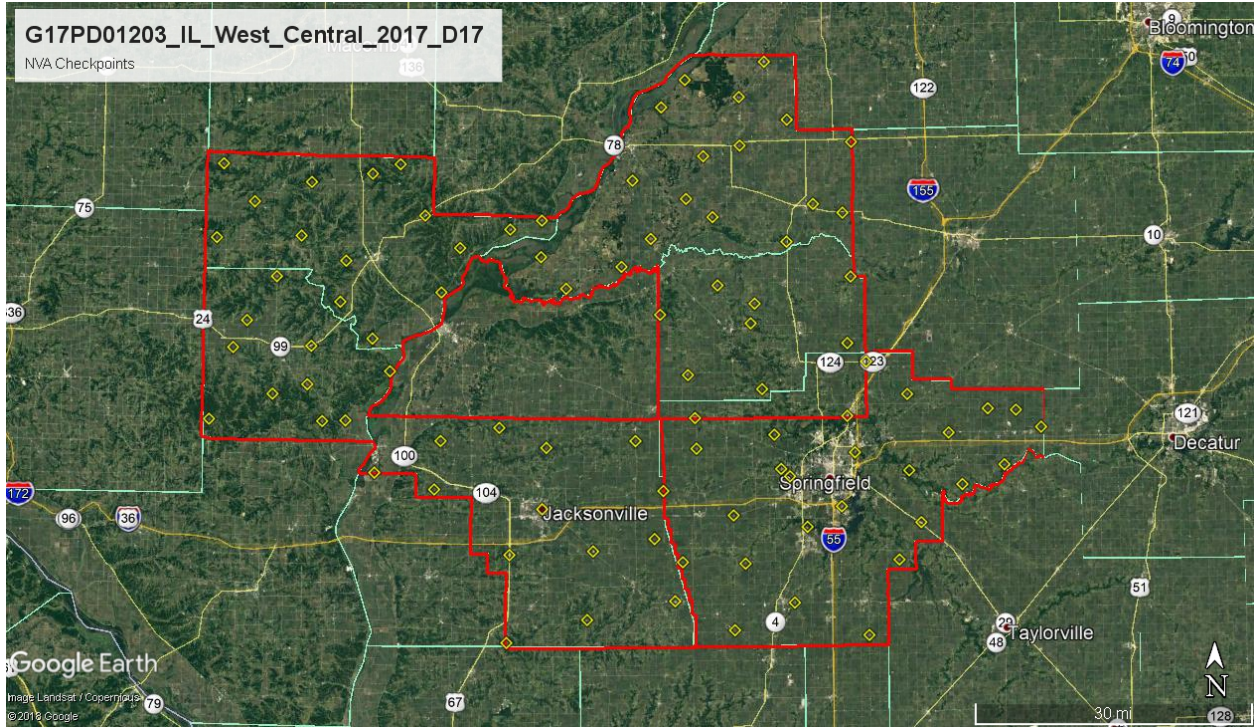
Figure 13 – Location of West Central LiDAR NVA Checkpoints
