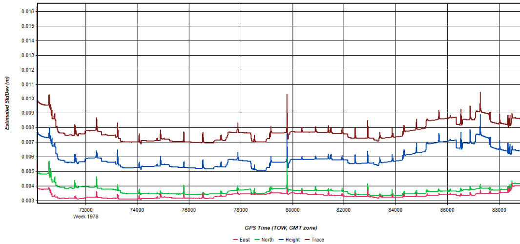
Figure 2: W_Central_3DEP_20171203_192639 [Smoothed TC Combined] - Estimated Position Accuracy Plot
