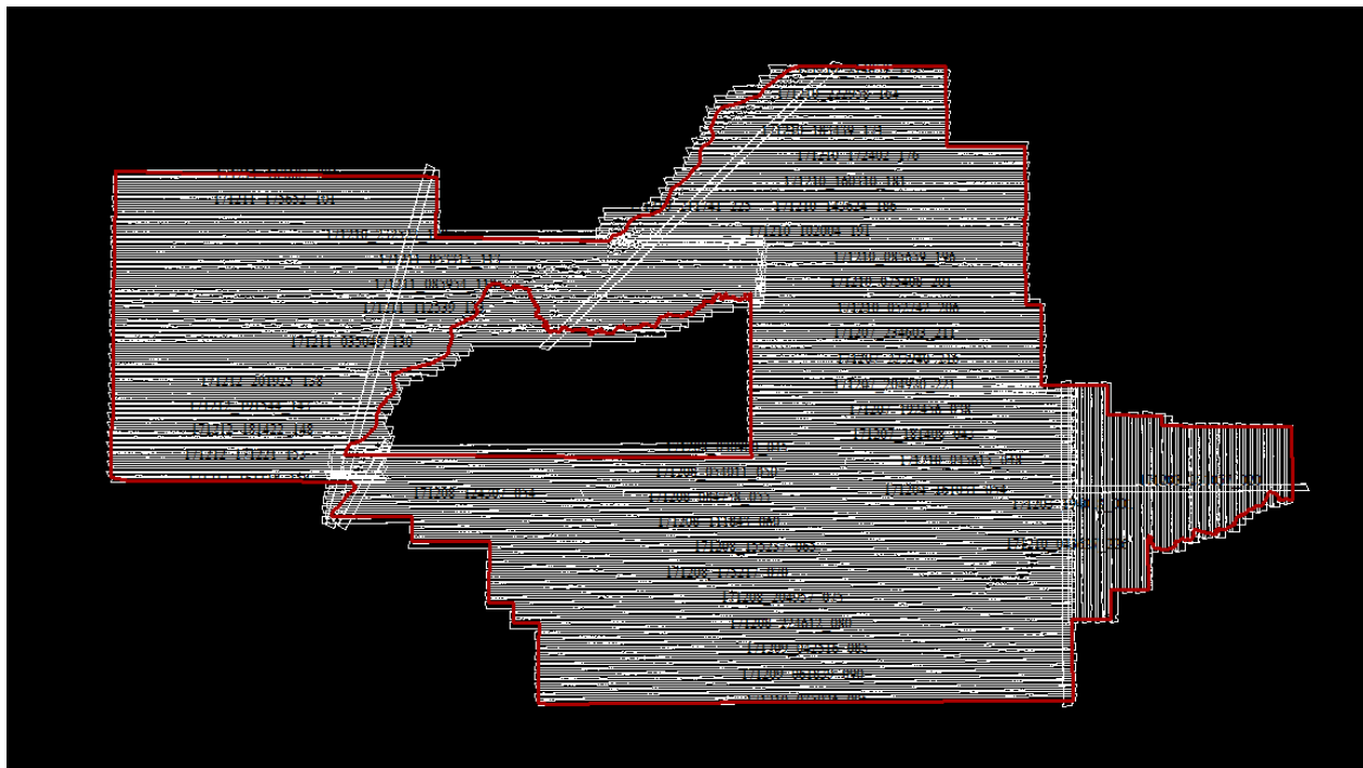
Figure 4 – Lidar swath coverage over AOI.
