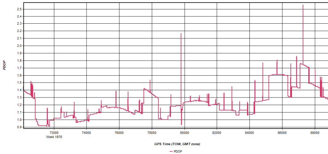
Figure 4: W_Central_3DEP_20171203_192639 [Smoothed TC Combined] - PDOP Plot
