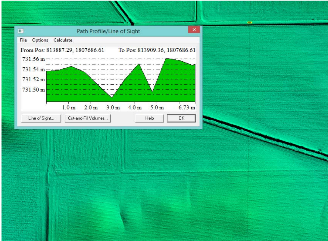
Figure 11 – The flight line ridge is less than 8 cm. Overall, the IL_West Central project data meets the project specifications for 8 cm RMSDz relative accuracy requirement.
