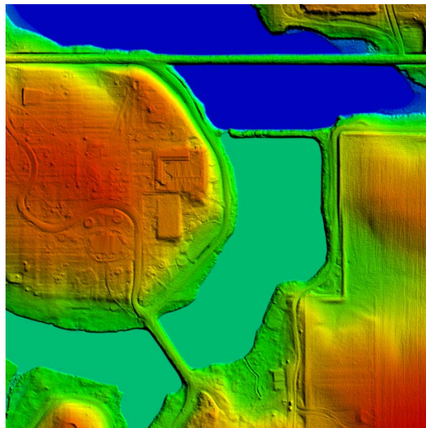
Figure 16 – IL_ West Central County project bare earth DEM
