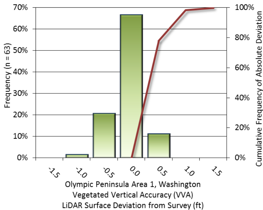
Figure 11: Frequency histogram for LiDAR surface deviation from all land cover class point values (VVA)
