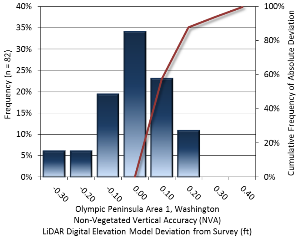
Figure 9: Frequency histogram for LiDAR DEM surface deviation from non-vegetated quality assurance point values
