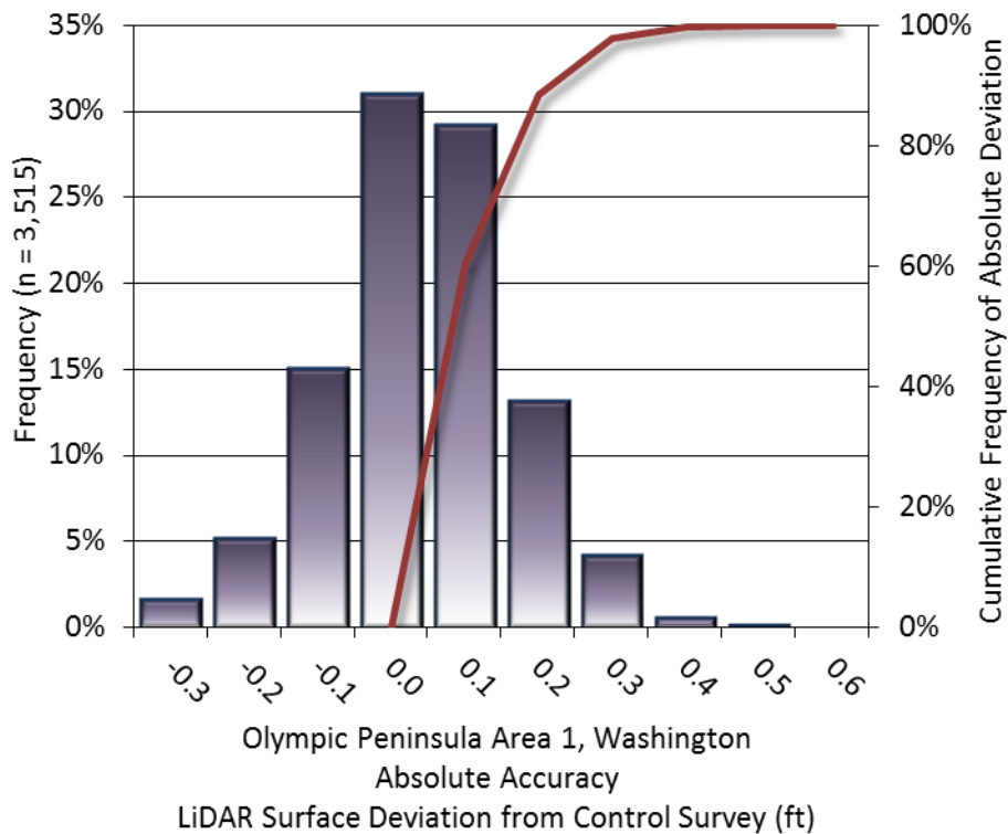
Figure 10: Frequency histogram for LiDAR surface deviation from ground control point values
