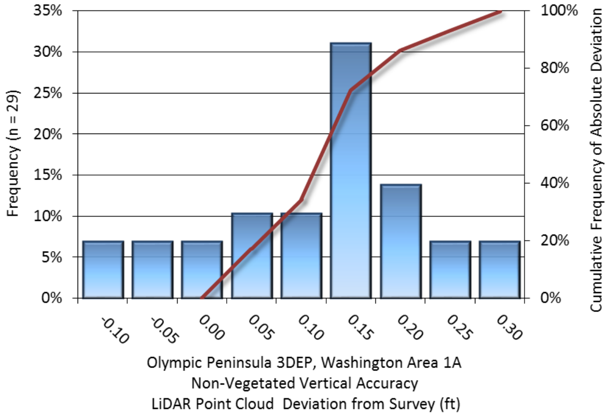
Figure 9: Frequency histogram for LiDAR unclassified point deviation from non-vegetated quality assurance point values
