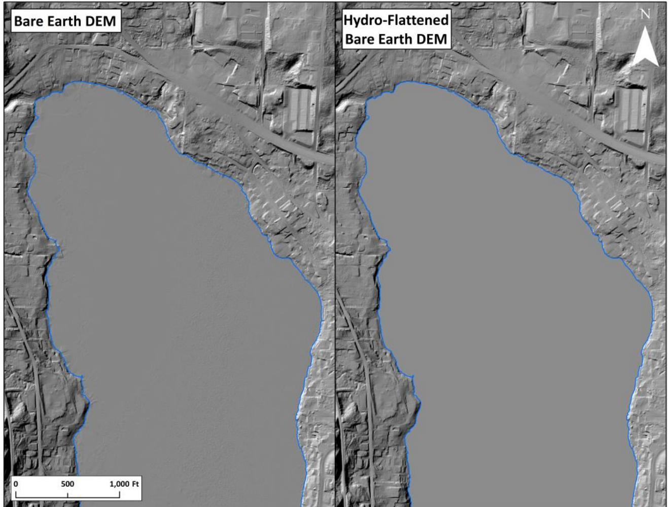
Figure 3: Example of hydroflattening in the Olympic Peninsula LiDAR dataset
