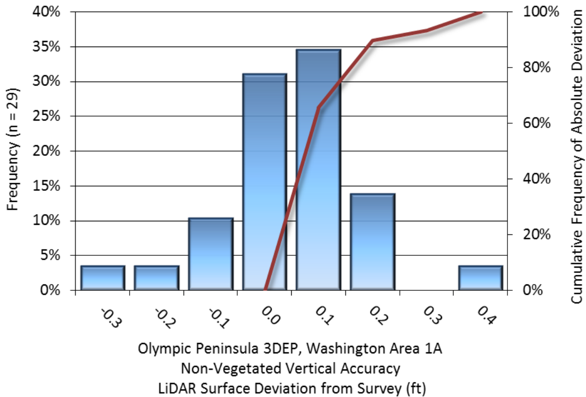
Figure 8: Frequency histogram for LiDAR DEM surface deviation from non-vegetated quality assurance point values
