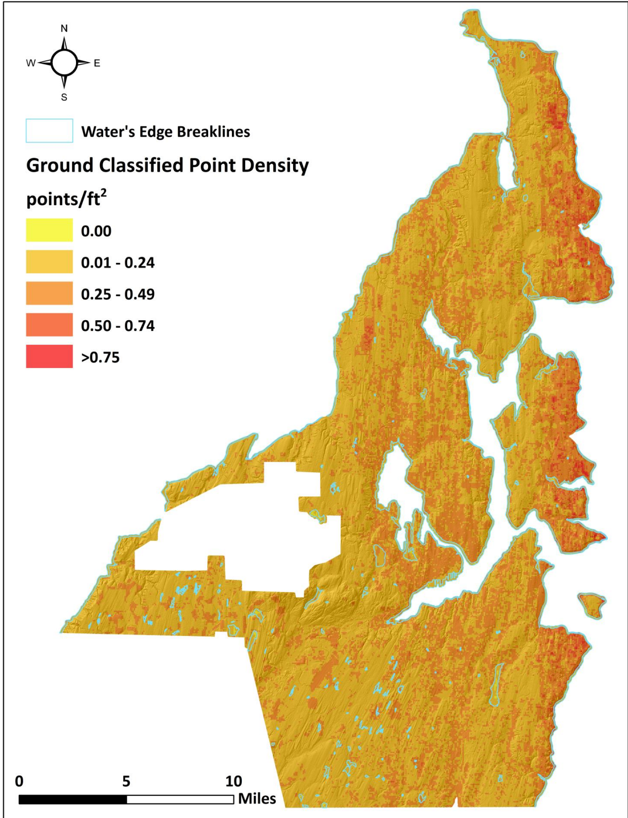
Figure 7: Ground classified point density map for the Olympic Peninsula site (100 m x 100 m cells)
