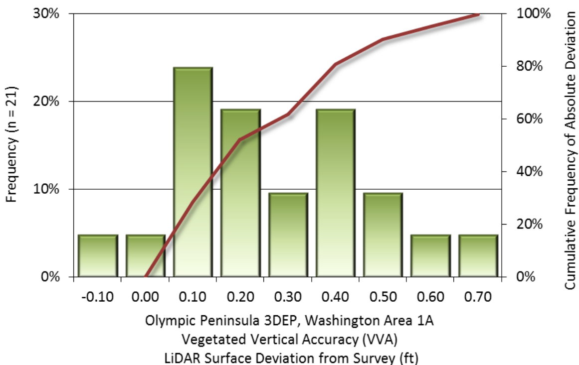
Figure 11: Frequency histogram for LiDAR surface deviation from all land cover class point values (VVA)
