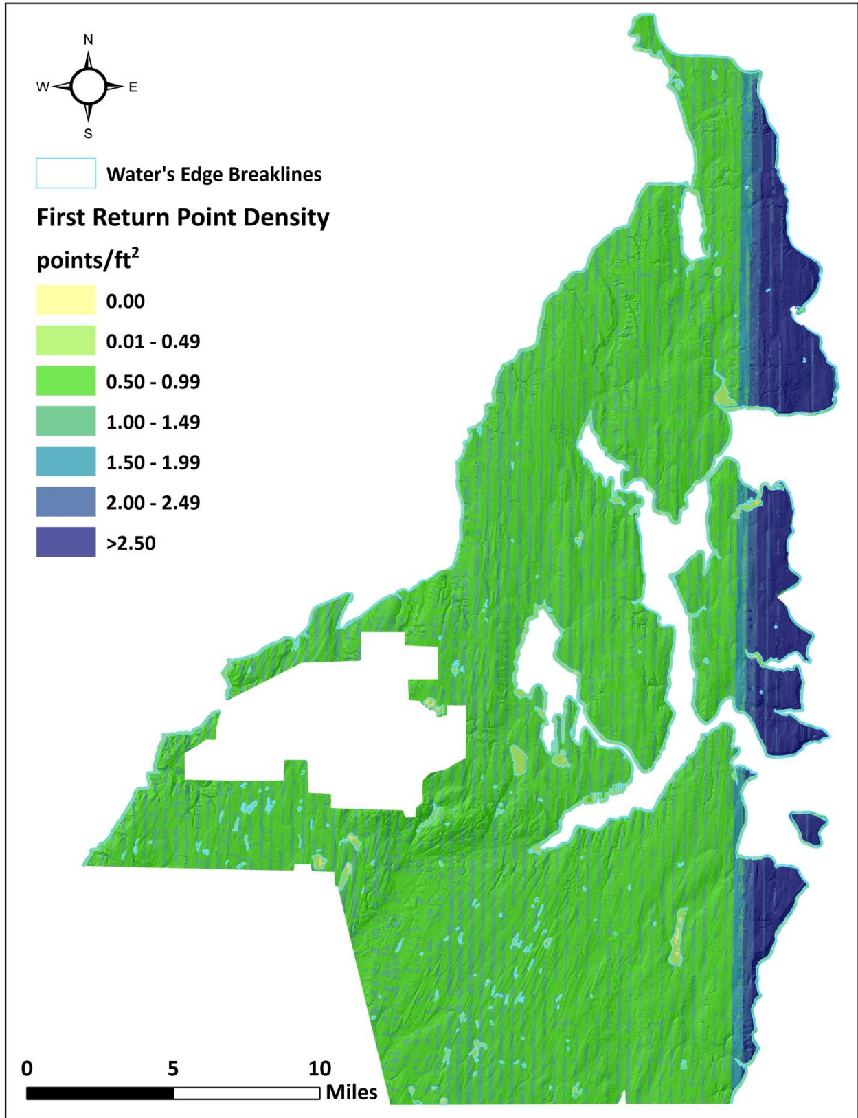
Figure 6: First return point density map for the Olympic Peninsula site (100 m x 100 m cells)
